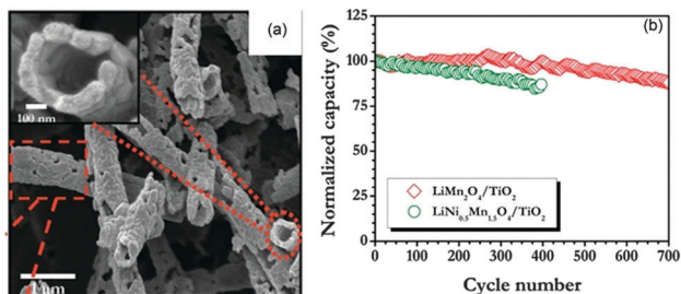
Fig. 10 (a) FESEM image of \text{LiMn}_2\text{O}_4 nanofibers. Inset: magnified view of nanofibers indicating a hollow structure. (b) Normalized capacity of \text{LiMn}_2\text{O}_4/\text{TiO}_2 (at a current density of 300 \text{ mA g}^{-1} ) and \text{LiNi}_{0.5}\text{Mn}_{1.5}\text{O}_4/\text{TiO}_2 (at a current density of 150 \text{ mA g}^{-1} ) full cells. Reproduced with permission from ref. 40. Copyright 2015, The Royal Society of Chemistry.
