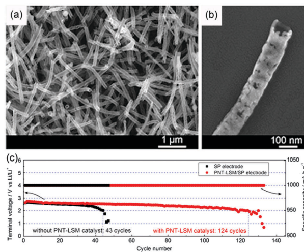
Fig. 11 (a and b) PNT-LSM after calcination at 650^\circ\text{C} for 3 h. (c) Voltage of the terminal discharge vs. the cycle number for Li- \text{O}_2 cells with and without a PNT-LSM catalyst at 0.15 \text{ mA cm}^{-2} . Reproduced with permission from ref. 44. Copyright 2013, Wiley-VCH Verlag GmbH & Co.
