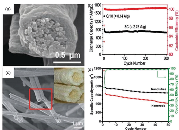
Fig. 9 (a) A cross-sectional SEM view of a single Si nanoparticles@C indicating that the core full of Si nanoparticles is wrapped by carbon shell. (b) Cycling performance of Si nanoparticles@C measured at 3C rate (2.748 A g -1 ), and the right axes are Coulombic efficiencies. Reproduced with permission from ref. 36. Copyright 2012, American Chemical Society. (c) FESEM image of CaSnO 3 nanotubes. The inset in (d) is a photograph of egg-roll. (d) Cycling performance of CSO-NT and CSO-NR at a current density of 60 mA g -1 . Reproduced with permission from ref. 37. Copyright 2013, The Royal Society of Chemistry.
