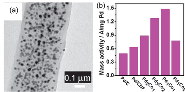
Fig. 8 (a) HRTEM of Pd x Co y /ECF nanocomposite. (b) Mass activity of Pd-based electro-catalysts for formic acid oxidation. Reproduced with permission from ref. 32. Copyright 2014, American Chemical Society.
