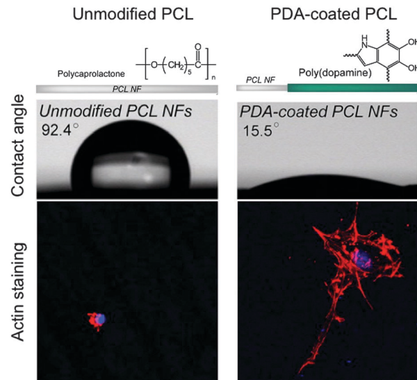
Fig. 5 Water contact angle and actin expression on unmodified and PDA-coated PCL nanofibres, respectively. In the presence of a PDA ad-layer, cells positively expressed actin. Reproduced with permission from ref. 19, Copyright 2010 Elsevier.
