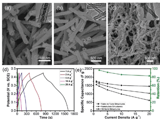
Fig. 12 (a–c) SEM images of \text{NiCo}_2\text{O}_4 tube-in-tubes, nanotubes and solid 1D nanostructures. The insets are their corresponding HRTEM images. (d) Galvanostatic charge/discharge profiles of \text{NiCo}_2\text{O}_4 tube-in-tube nanostructures at various current densities in a 2.0 M \text{KOH} electrolyte. (e) The specific capacitance at various current density of \text{NiCo}_2\text{O}_4 tube-in-tube, nanotube, and 1D solid nanostructures. Reproduced with permission from ref. 10. Copyright 2015, American Chemical Society.
