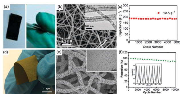
Fig. 13 (a) Photograph of electrospun carbon nanofibres (left) and the folded state (right). (b) SEM and HRTEM images of the carbon nanofibres. (c) Cyclic stability of a carbon electrode at a current density of 10 \text{ A g}^{-1} . Reproduced with permission from ref. 46. Copyright 2015, American Chemical Society. (d) Photograph of the flexible \text{V}_2\text{O}_5/\text{CNF} film. (e) Low magnified and high magnified SEM (inset) of \text{V}_2\text{O}_5/\text{CNF} film. (f) The specific capacitance of \text{V}_2\text{O}_5/\text{CNF} at various current densities. (g) Cycling stability of the flexible \text{V}_2\text{O}_5/\text{CNF}/\text{CNF} solid SC device at a current density of 1.2 \text{ A g}^{-1} . The inset shows galvanostatic charge-discharge voltage curves for the last ten cycles. Reproduced with permission from ref. 47. Copyright 2015, Wiley-VCH Verlag GmbH & Co.
