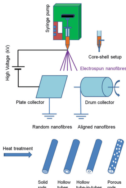
Fig. 2 Schematic of an electrospinning setup to obtain random, aligned nanofibres and nanofibres with various structures, which are influenced by the properties of precursor polymers, electrospinning parameters, and post-treatment.
