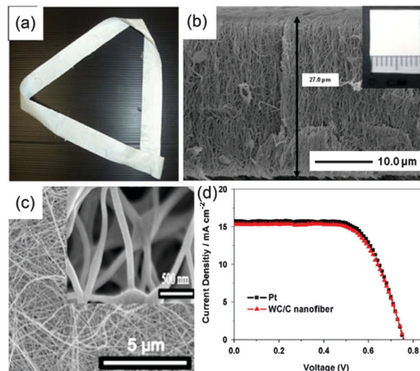
Fig. 7 (a) Photo image of horizontally aligned electrospun TiO 2 nanofibrous ribbon. (b) SEM image of vertically aligned electrospun TiO 2 nanowires. The inset is the photo image of the aligned nanofibrous film indicating size reduction after sintering. Reproduced with permission from ref. 27. Copyright 2011, The Royal Society of Chemistry. (c) SEM image of electrospun WC/C composite. (d) Photocurrent–photovoltage characteristics for QDSCs with different materials as the counter electrodes. Reproduced with permission from ref. 30. Copyright 2014 Elsevier.
